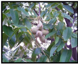
Butternut (16SrVII-A)
